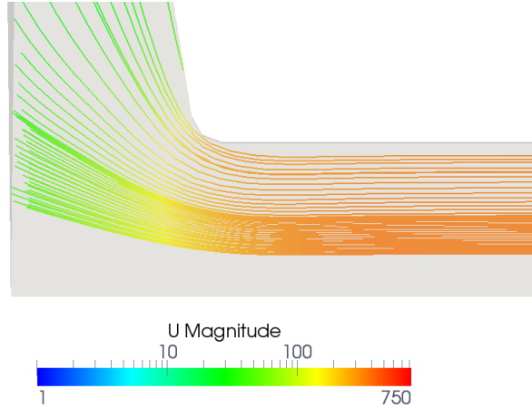
Figure 6.3. Vena-contracta experienced at nozzle inlet.
